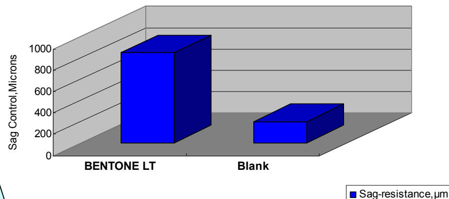
Sag-resistance, Microns, Original Waterborne Protective Coatings Primer
