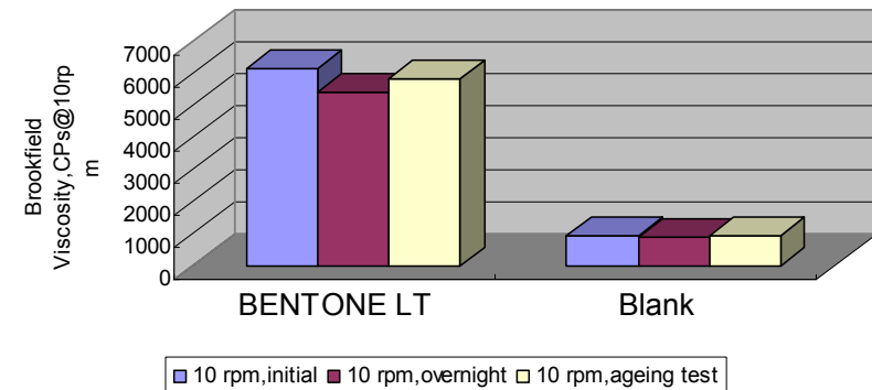
Brookfield Viscosity, CPs@10rpm, In Waterborne Protective Coatings Primer
