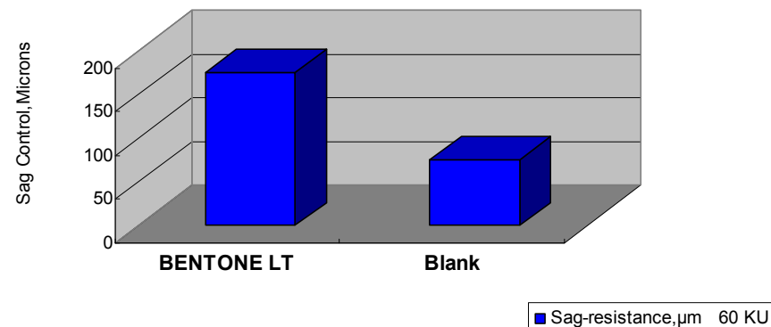
Sag resistance, Microns, ,in Waterborne Protective Coatings Primer
