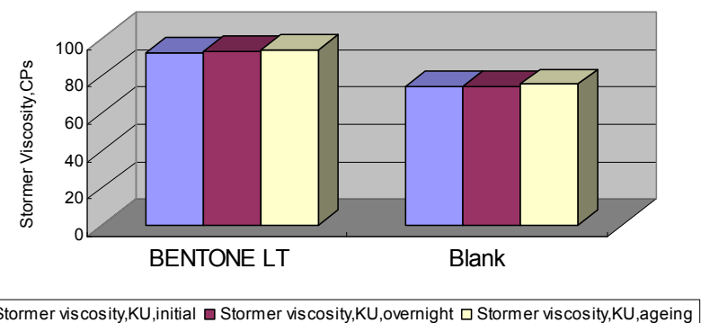
Stormer Viscosity, KU in Waterborne Protective Coatings Primer
